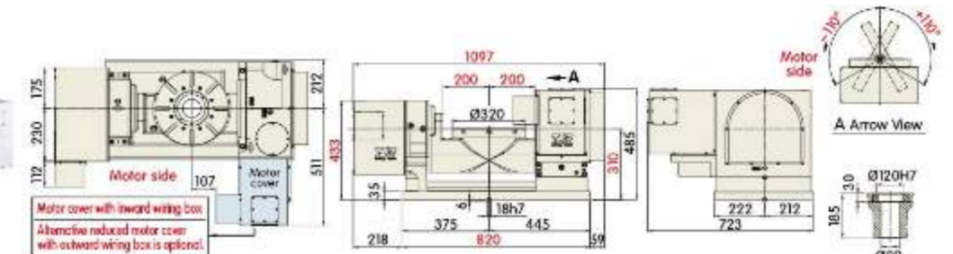
Drawing of Control Hole
