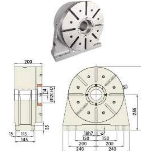
RT-170F (Without Brake)
