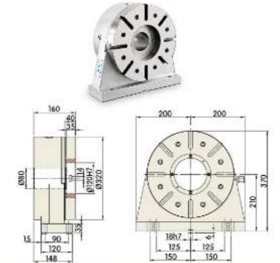
RTH-400A (Hydraulic 115 kgf-m)
