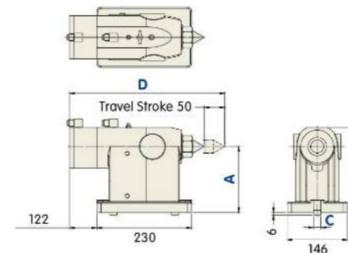
▲ ATTJ-210 (with Pneumatic switching valve)
