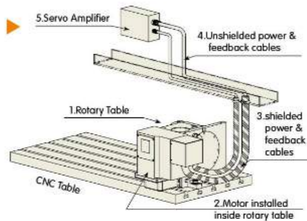
Drawing ⑥ 5 main components of the 4 th axis
