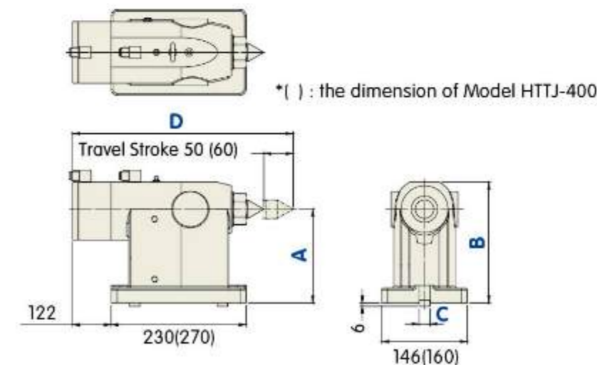
▲ HTTJ-320 (with Hydraulic switching valve)
