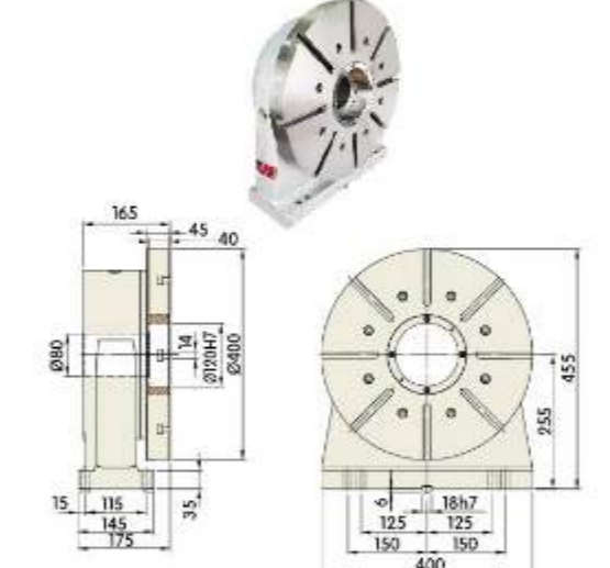
RT-135 (Without Brake)
