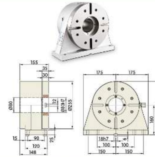
RTH-400 (Hydraulic)
