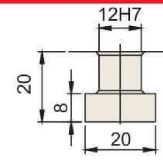
T-Slot Dimension
