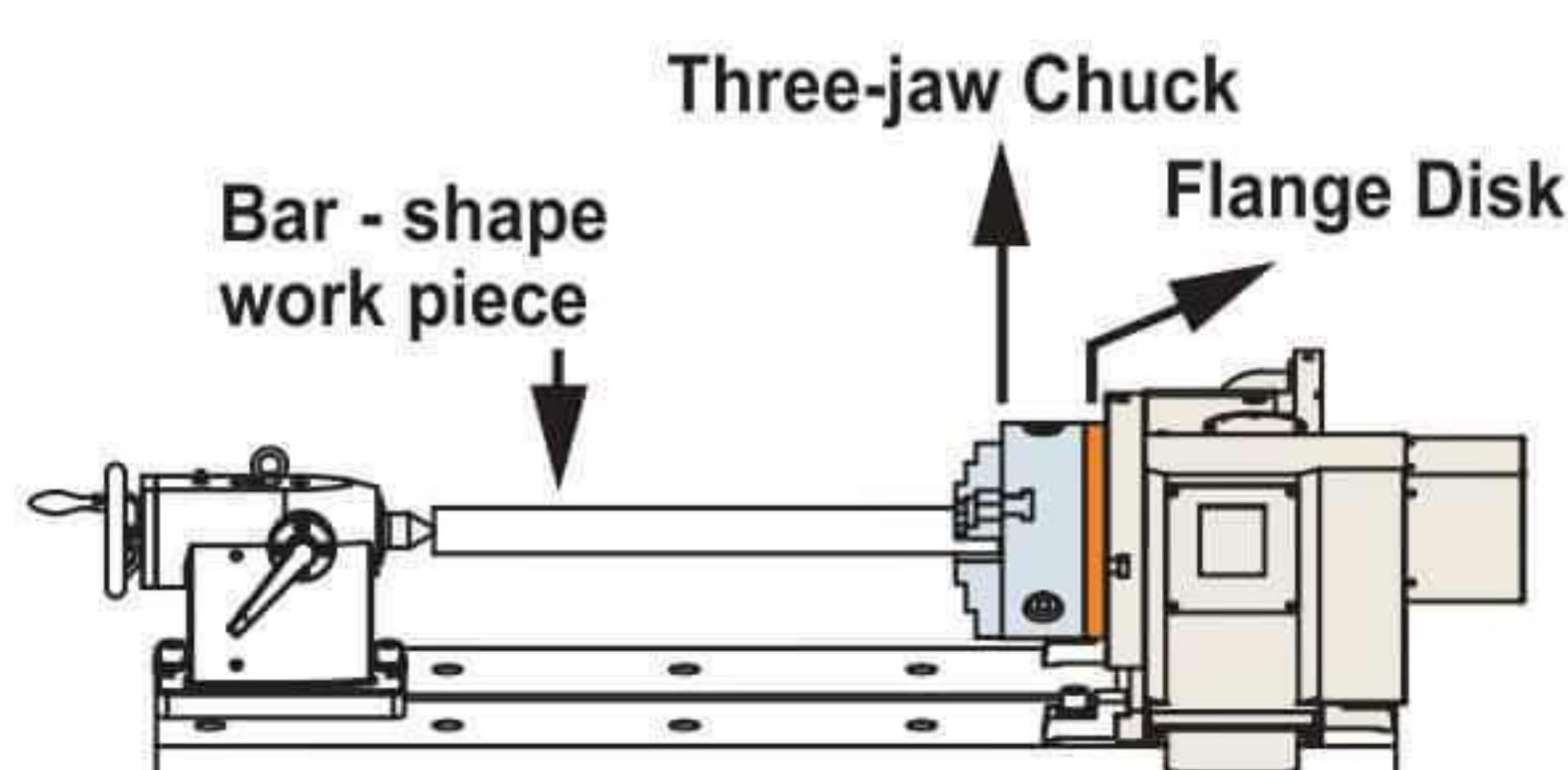
▲ Diagram of Chuck Installation
