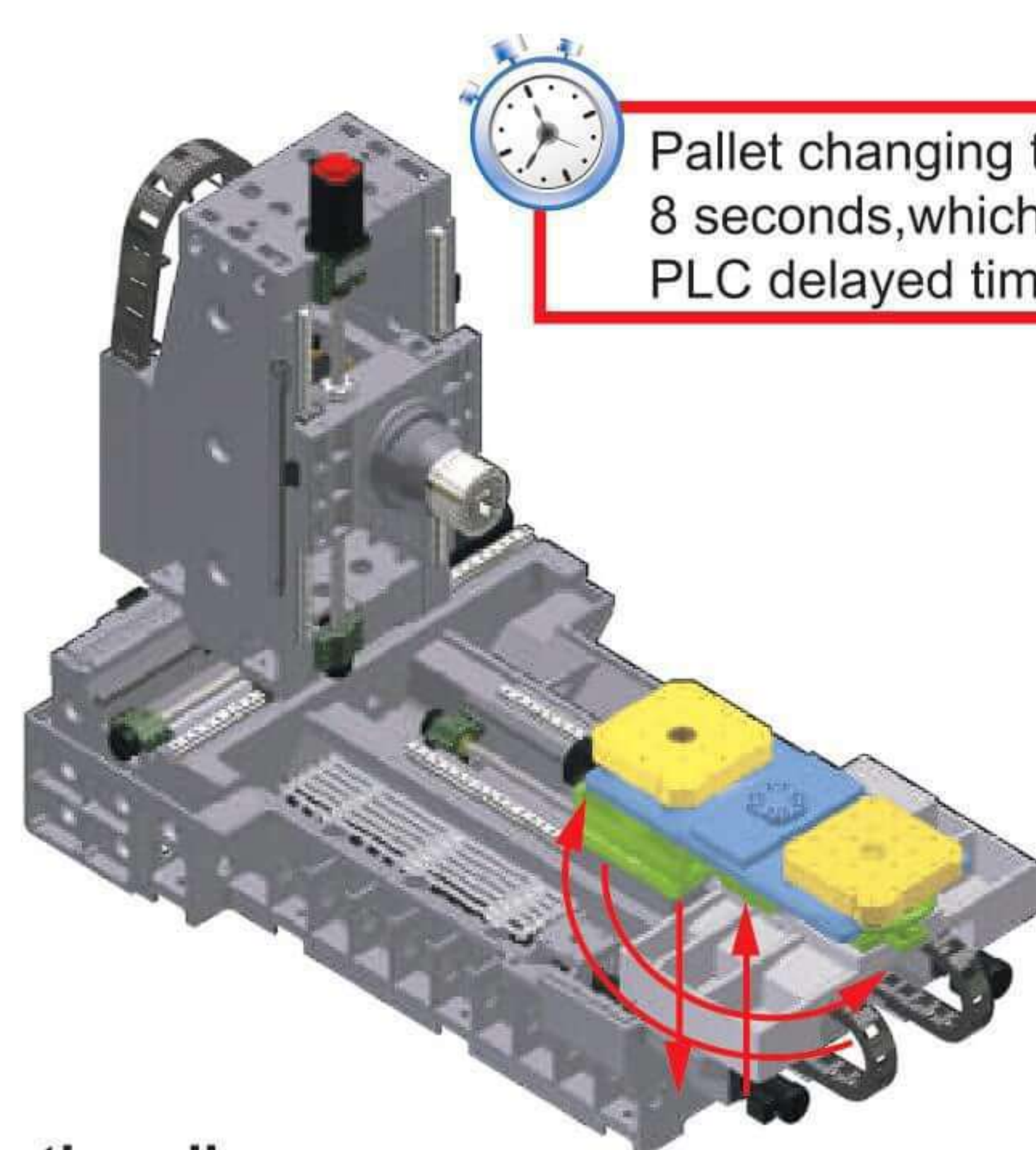
▲ CTH-630 (tray type APC)
