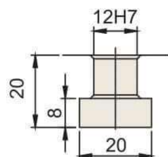
T-Slot Dimension
