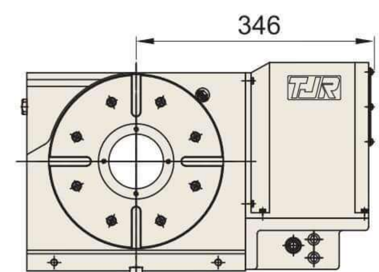
▲ Drawing ③-1 : HR-255N
