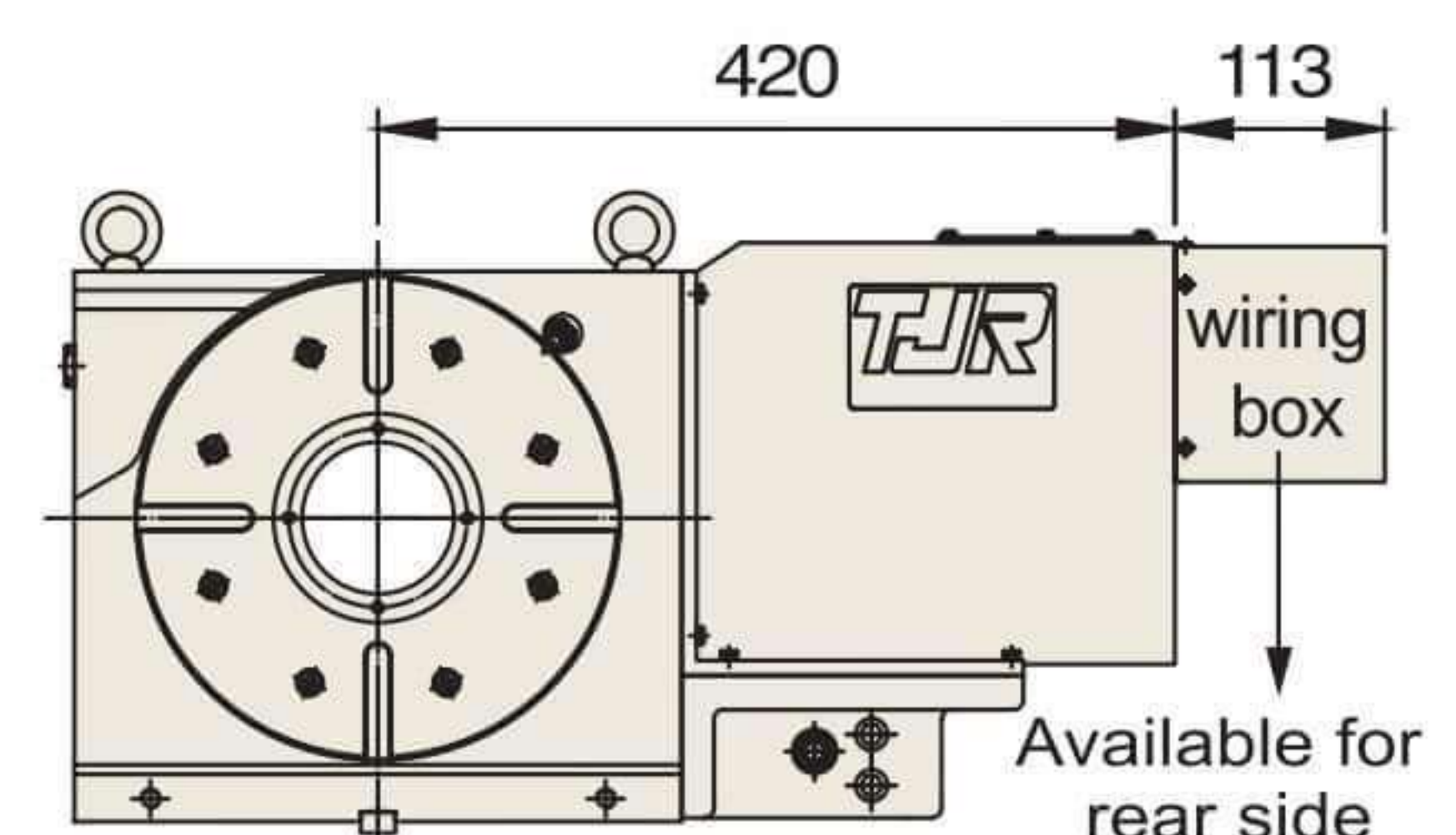
▲ Drawing ③ : HR-255R
