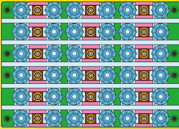
▶ Little King Kong Vise: An example of fixing round work-piece.
