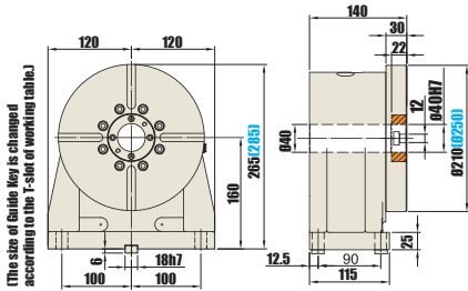
( ): When the faceplate is enlarged to ø250mm. Weight : 35kg
